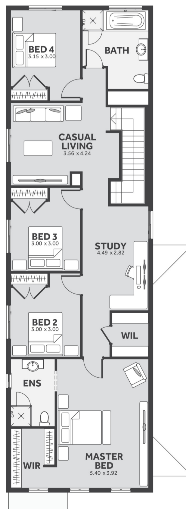
First Floor
