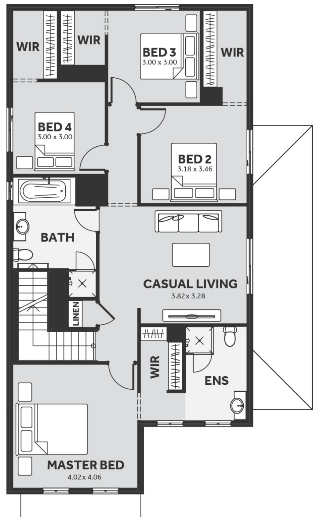
First Floor
