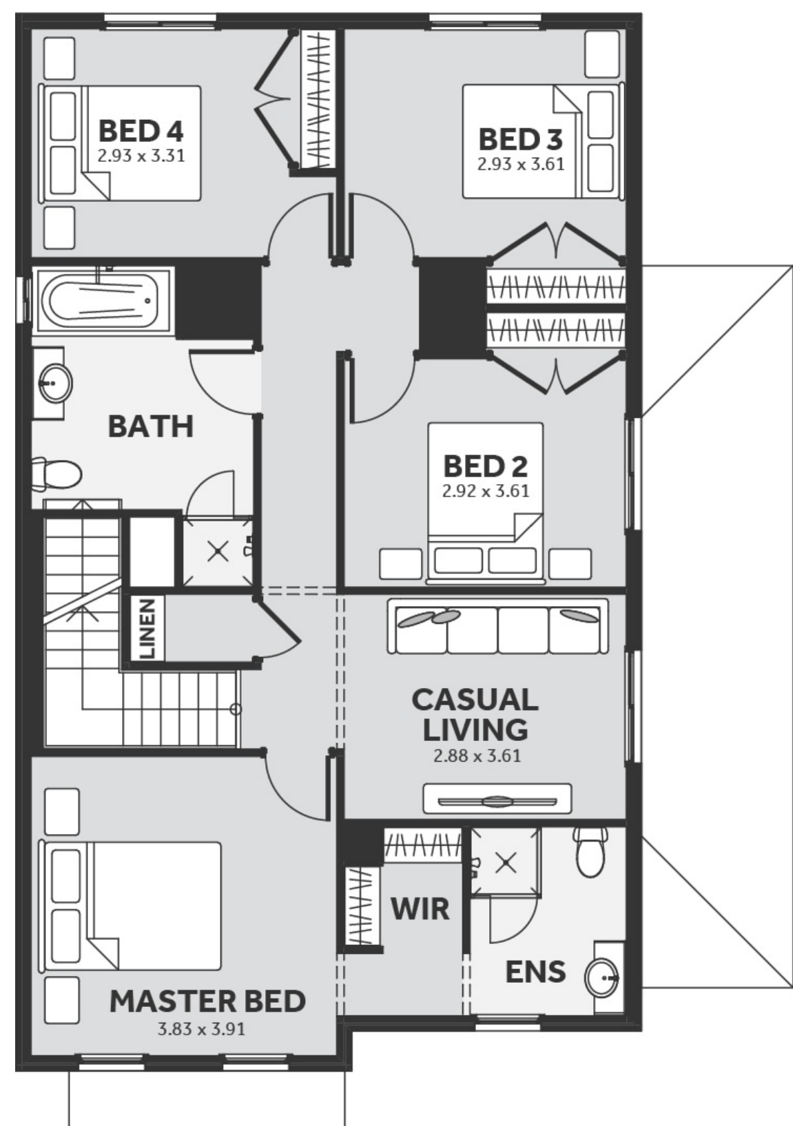
First Floor
