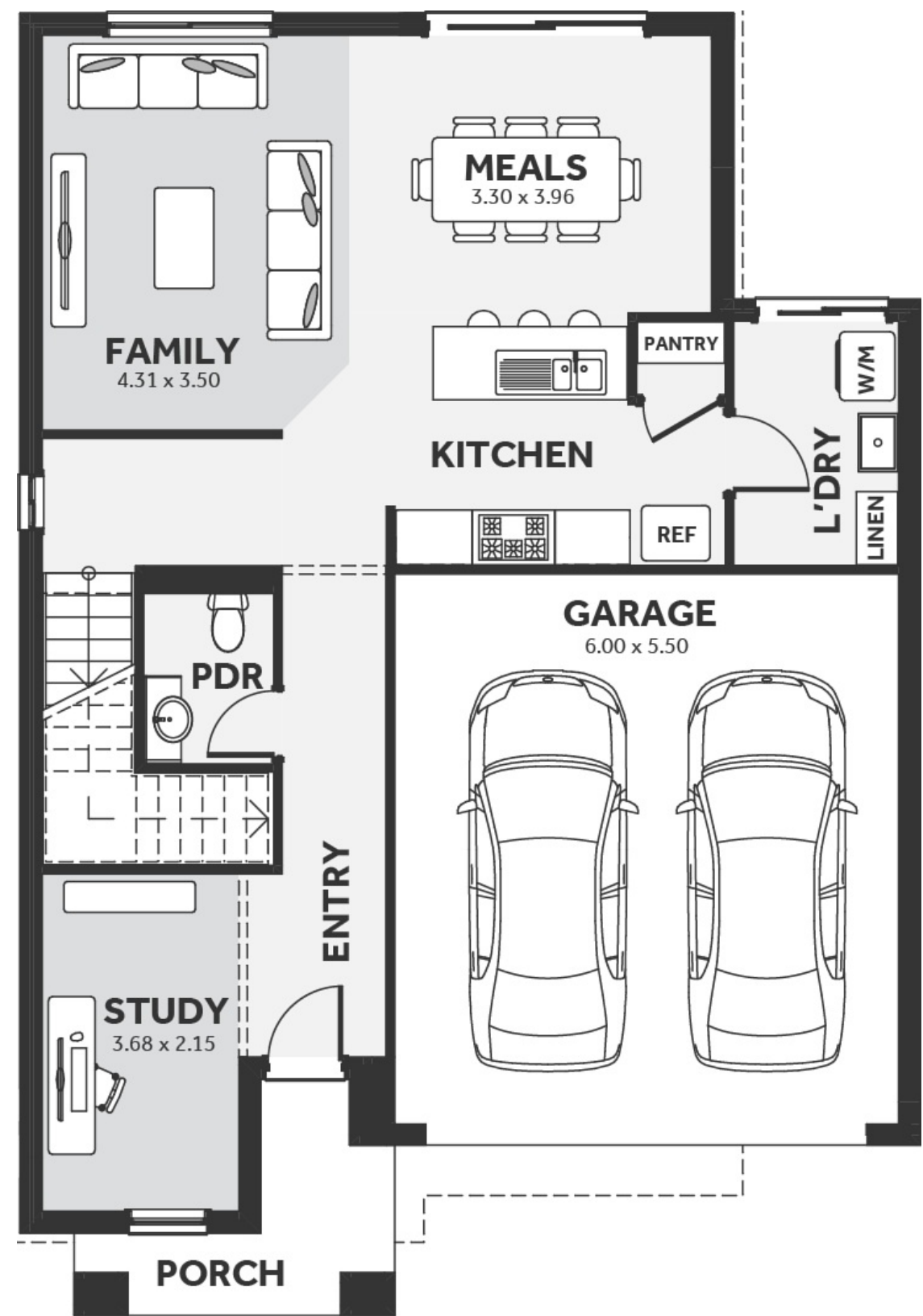
Ground Floor
